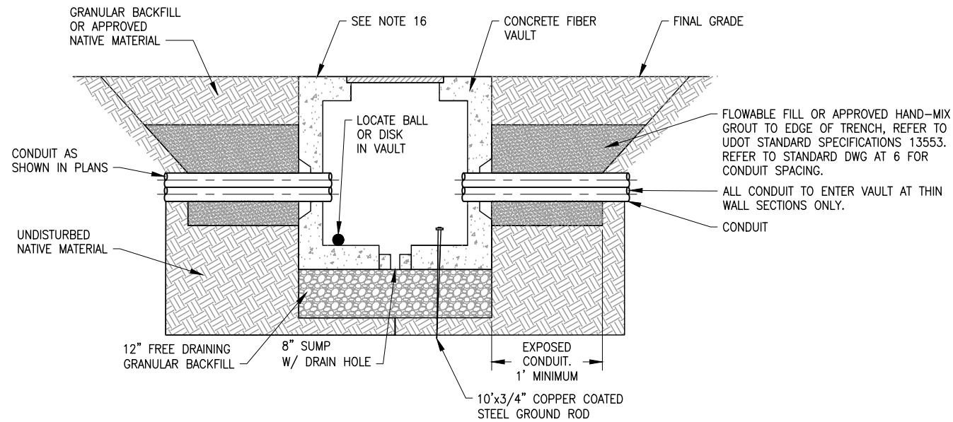
VAULT DIMENSIONS
