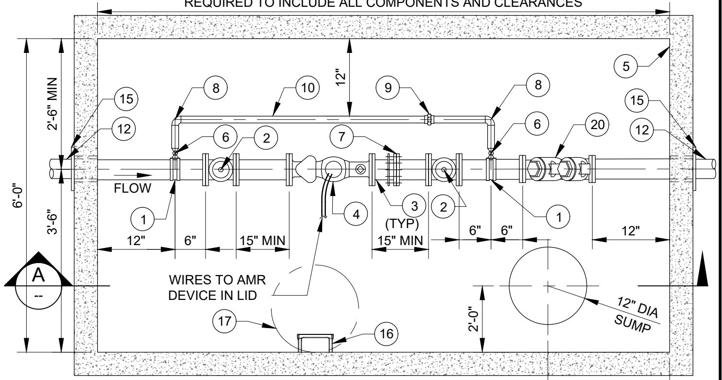
PLAN NTS
