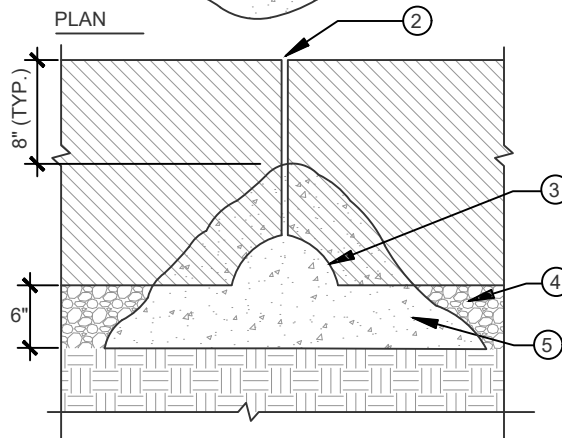
6 GRANITE CURB - SECTION NTS
