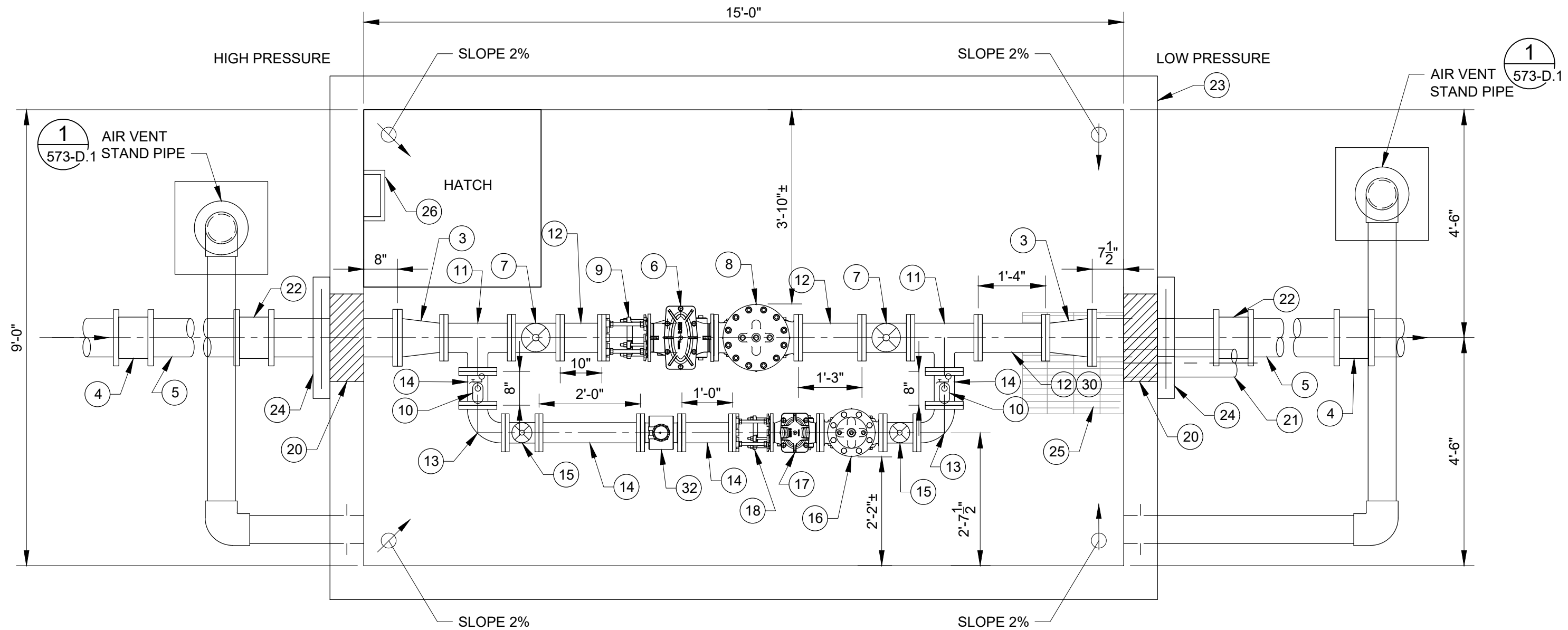
BASIC VAULT - PLAN VIEW SCALE: 1/2" = 1'-0" 1 0 2 4 SCALE IN FEET
