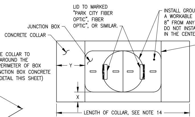
PLAN VIEW-JUNCTION BOX AND CONCRETE COLLAR SCALE: NONE
