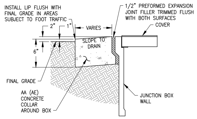
JUNCTION BOX CONCRETE COLLAR DETAIL SCALE: NONE
