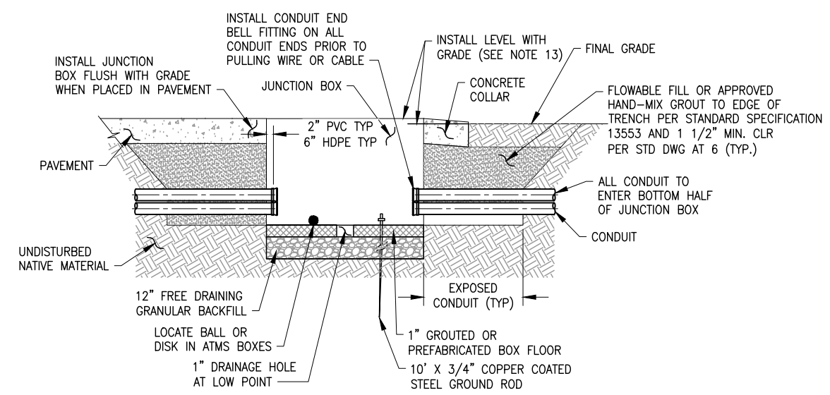
JUNCTION BOX CONDUIT PENETRATION DETAIL SCALE: NONE
