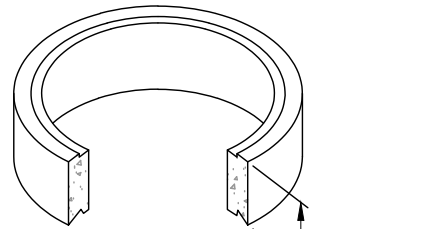
3/8" DIAMETER THREADED INSERT CAST IN RING AND COVER CONCRETE RISER AS REQUIRED
