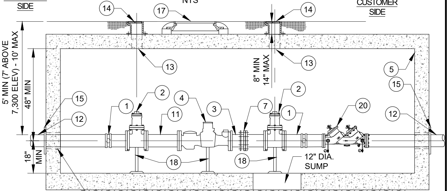
SECTION NTS
